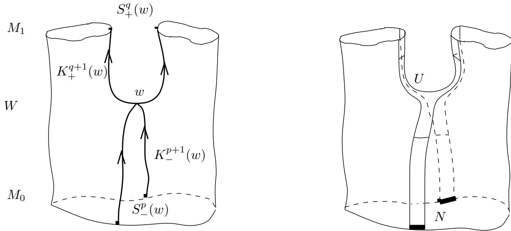
FIGURE 1. Trajectory disks of the critical point w contained inside a disk U
