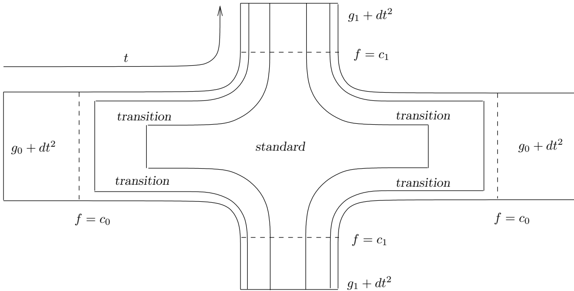
FIGURE 2. The metric \bar{g} on the disk U
