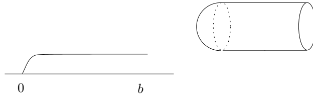
FIGURE 3. A torpedo function and the resulting torpedo metric
