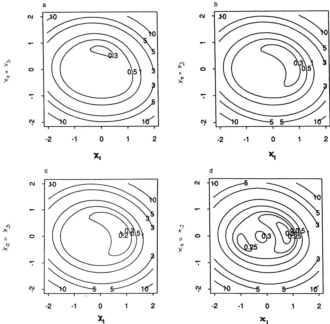
Figure 3. Successive Variance Contours as Points Are Added Sequentially to the Design of Table 4: (a) Original Design, N = 16 , Q^* = .9710 ; (b) Points 1-17, N = 17 , Q^* = .9855 ; (c) N = 18 , Q^* = .9899 ; (d) N = 19 , Q^* = .9918 .
