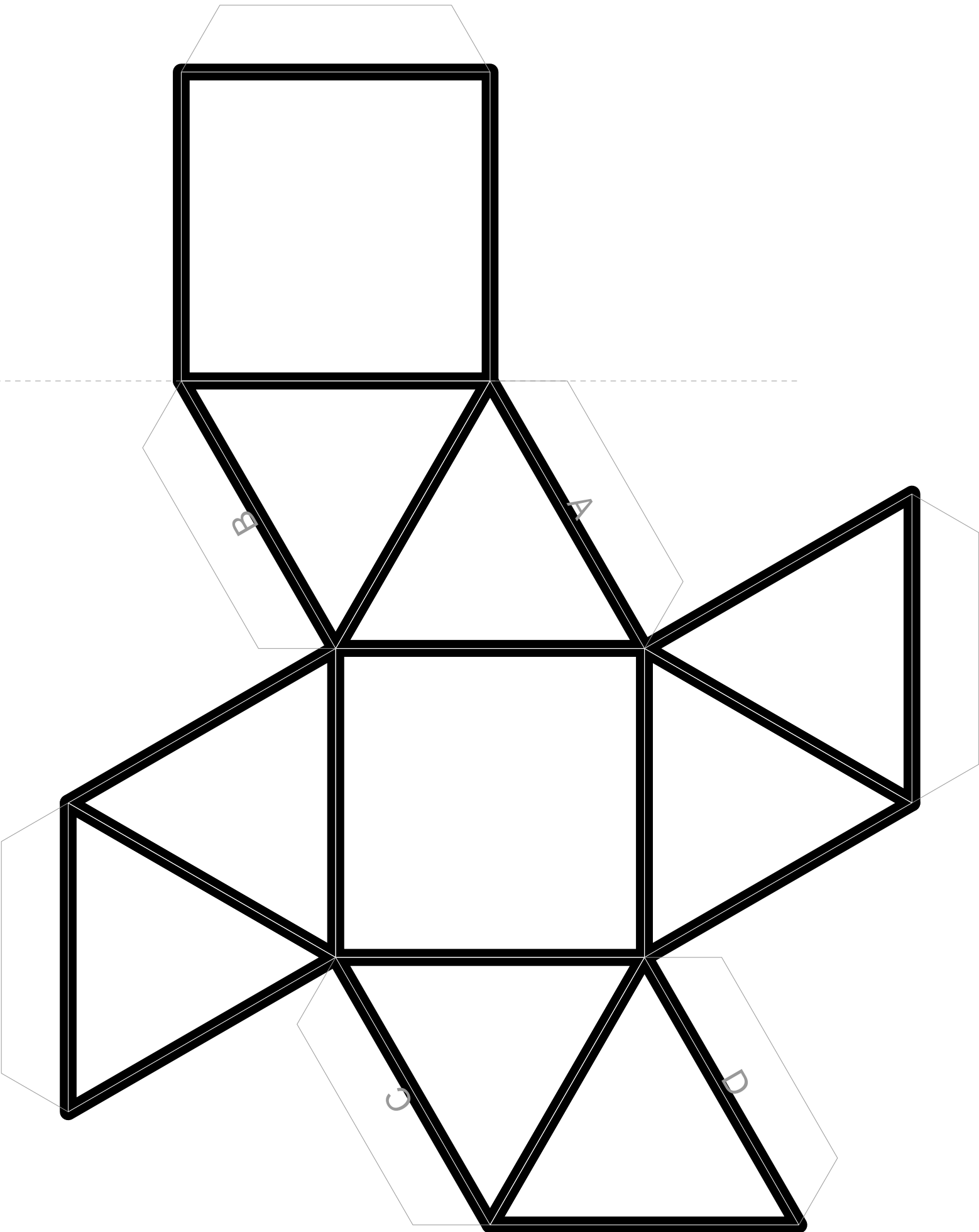
Tetra-Antiprisma (3,3,3,4)
