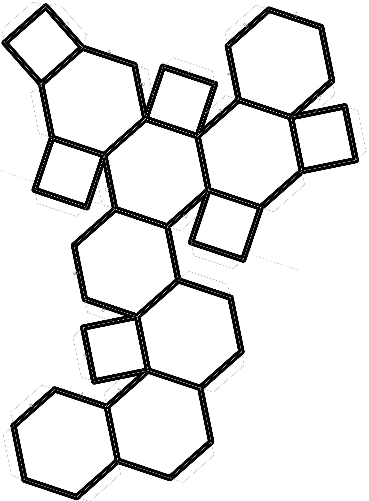
Stutz-Oktaeder (4,6,6) ( max. Kante = 3.0 cm )
