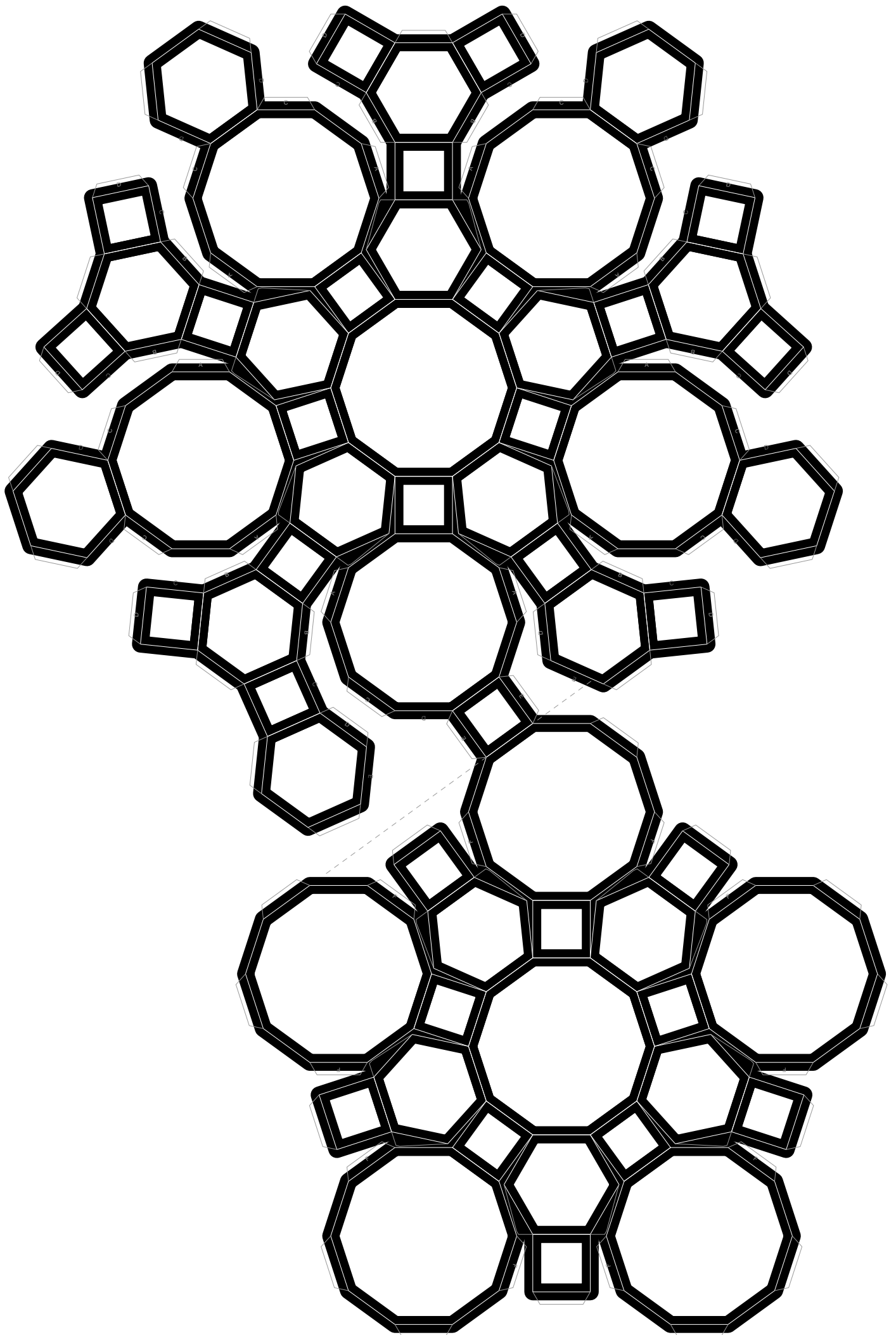
Gross-Rhombikositodekaeder (4,6,10) ( max. Kante = 1.2 cm )
